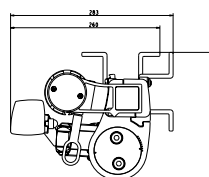
FA42 takmontering.
